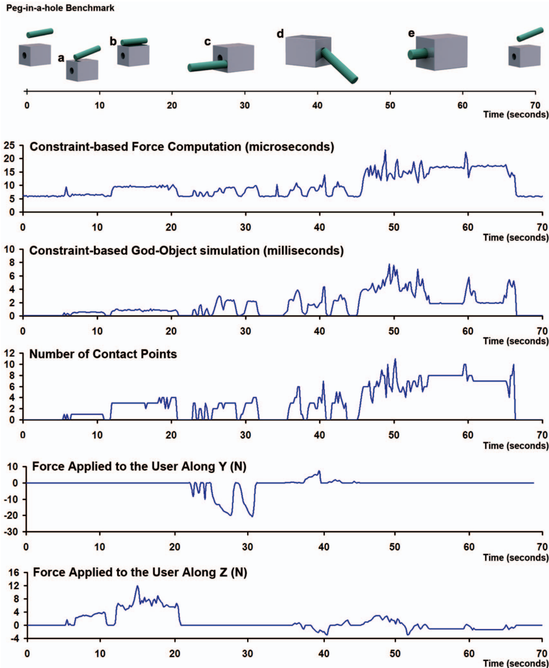
Fig. 11. Performance of our approach in the peg-in-a-hole benchmark. Our method computes a constraint-based force within a few microseconds , while a peg configuration update requires only a few milliseconds , which is sufficient to prevent visual lag in the simulation. As expected, the user feels a force in the Y direction only when he pushes the peg on the left side of the box (step c) or explores the right extremity of the hole (step d). Note how the combination of the collision detection and constraint-based quasi-statics algorithms tend to limit the number of simultaneous contact points during the interaction.
