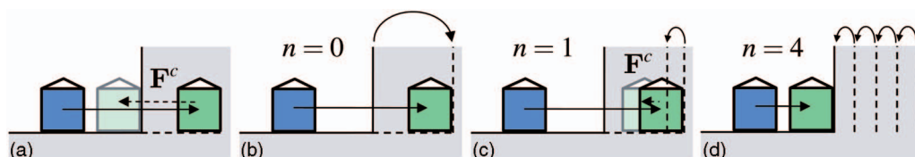
Fig. 6. Constraints adaptation. When a new constraint (here, a vertical plane) appears that would create too large a constraint force, it is first translated so that the constraint is satisfied by the current haptic device configuration, then progressively returned to its initial position. This helps us smooth the force felt by the user, while ensuring that small discontinuities signaling new contact points are felt.
