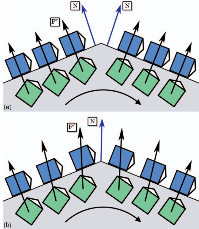
Fig. 8. Smoothing Effect. (a) The edge is felt because of the discontinuous force implied by the change in the normal direction. (b) Thanks to the use of the vertex normal N , the force shading method avoids the discontinuity and smoothes the edge.
