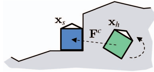
Fig. 2. Six degree-of-freedom god-object. Although the haptic device penetrates the environment obstacles (configuration x_h ), the god-object is constrained to remain on the surface of the obstacles (configuration x_s ). We propose new algorithms to compute the motion of the god-object and the force applied to the user based on the discrepancy between these two configurations.
