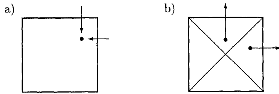
Figure 2: Generation of contact forces using volumes (the small dot represents the haptic interface point). a) Two possible paths to reach the same location in a square are shown; without a history we do not know which path was taken. b) Vector field method (in 2 dimensions): subdivide the square's area and assume that the user entered from the closest edge. The force vectors are normal to the edge and proportional to distance penetrated. This method is easily expanded to 3 dimensions.
